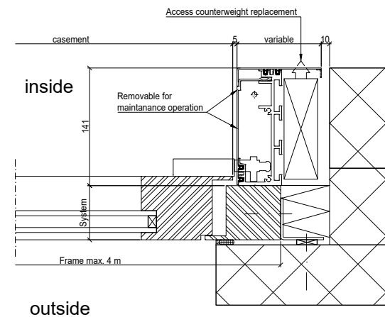
Horizontal section
