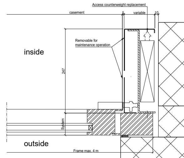
Horizontal section
