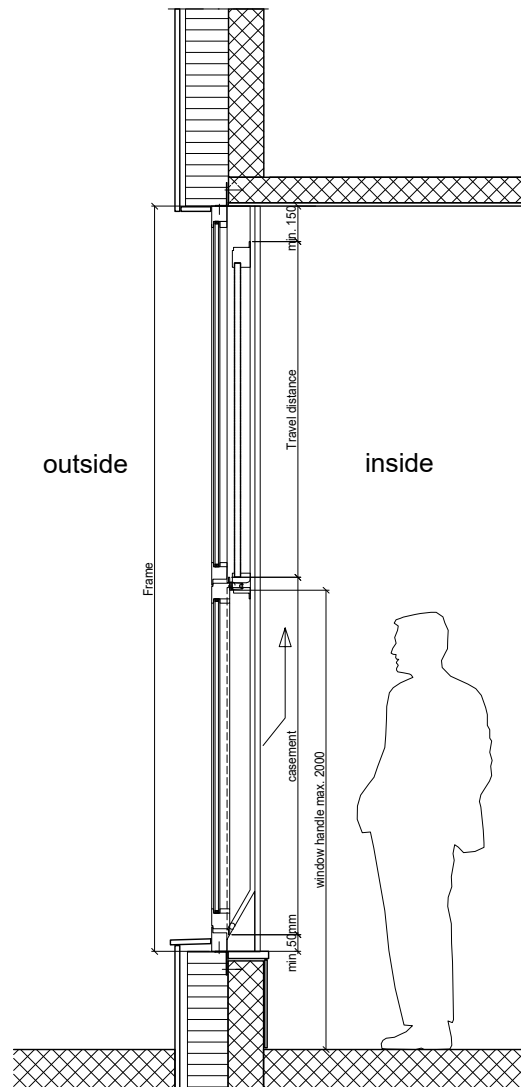
Vertical section
