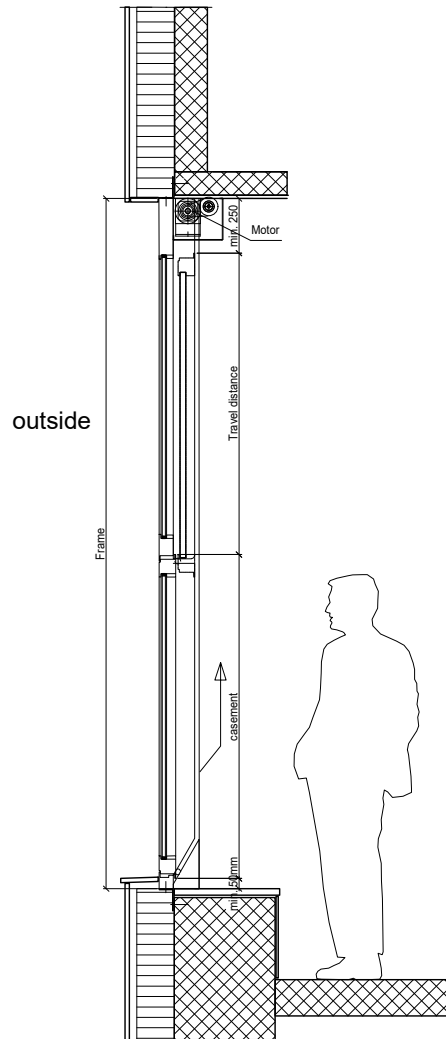
Vertical section
