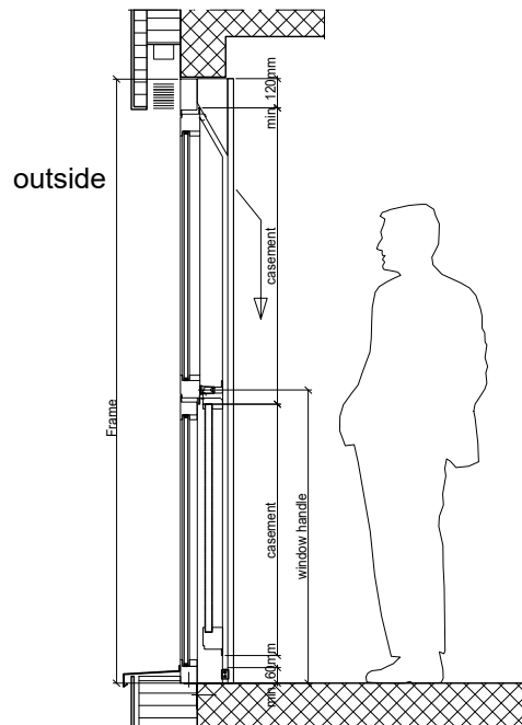
Vertical section
